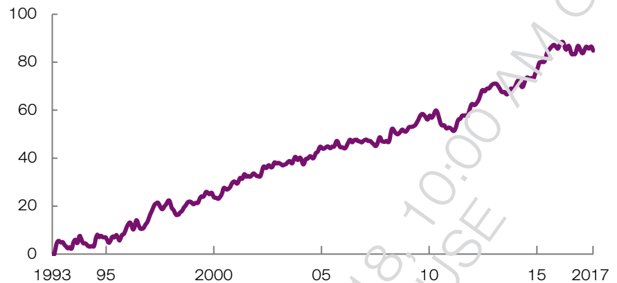
Mean sea level rise, 1993-2017, millimeters
